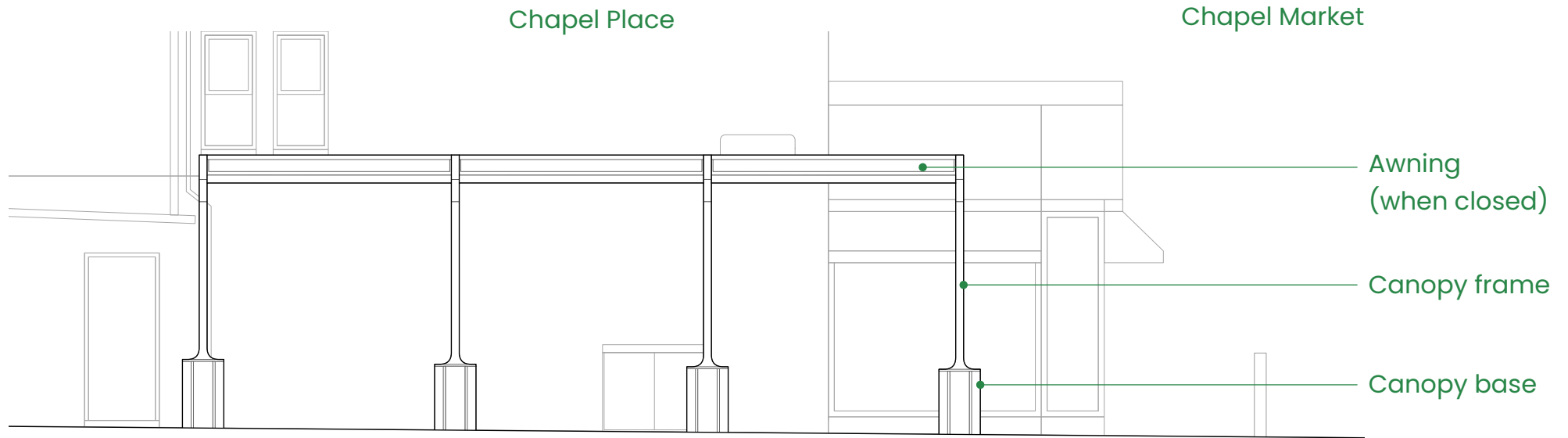
Chapel Market Canopy - West Elevation when closed
