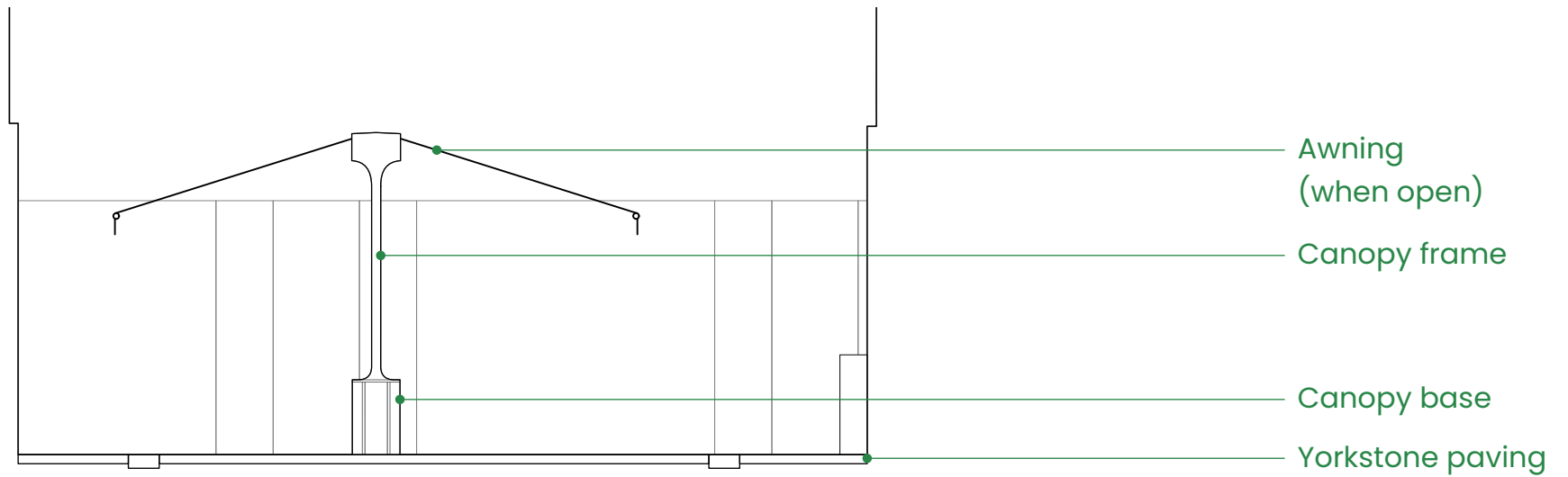
Chapel Market Canopy - South Elevation when open
